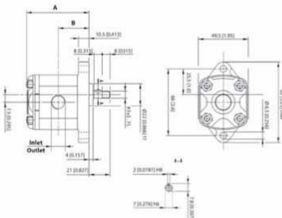
TFP0NN dimensions
