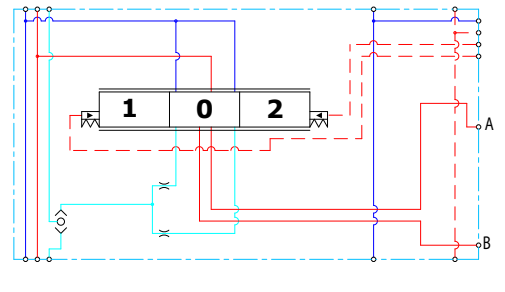
Uncompensated PVB with T0
