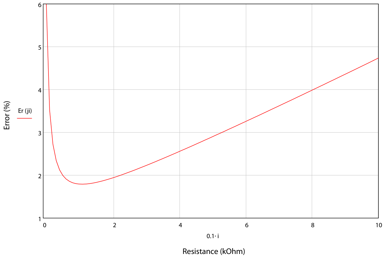
Resistance versus maximum measurement error
