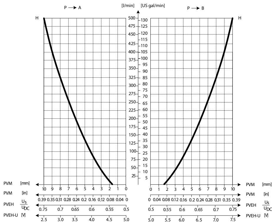
Oil Flow as Function of Spool Travel
