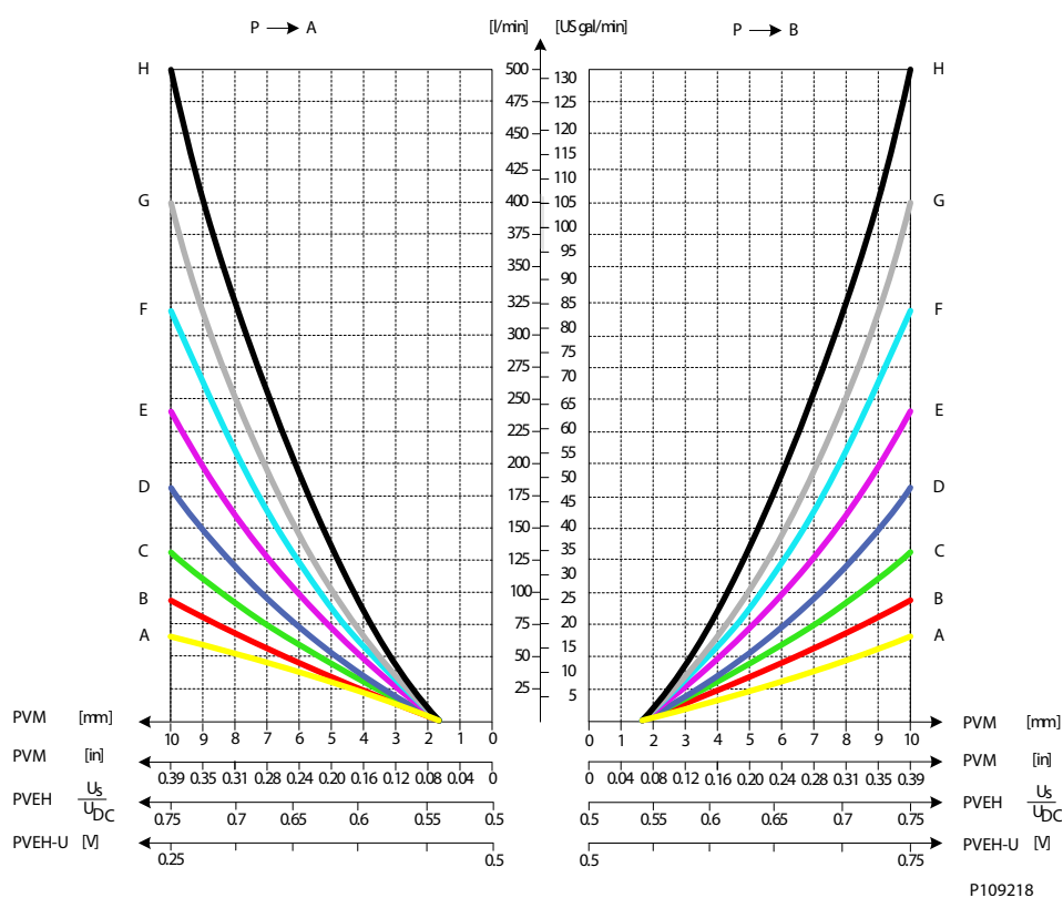
Oil Flow as Function of Spool Travel
