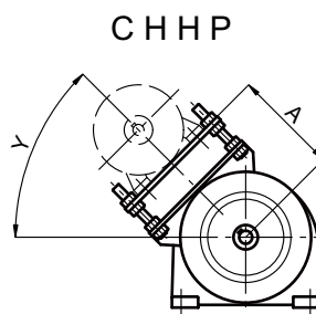
Motor at the left seen from high speed shaft
