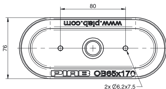
2x Ø6.2x7.5
