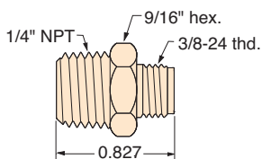
Part No. MIQC-VMQ Description 1/4" NPT Male, 3/8-24 Thd.
