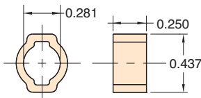
Part No. Description 5000-1 Hose Clamp
