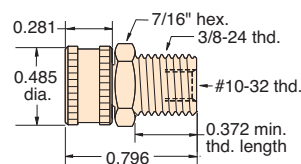
Part No. MIQC-CPF Description 3/8" Thread
