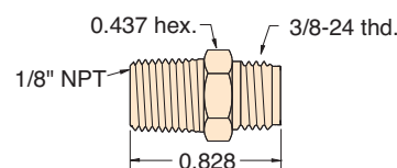
Part No. MIQC-VMP Description 1/8" NPT Male, 3/8-24 Thd.
