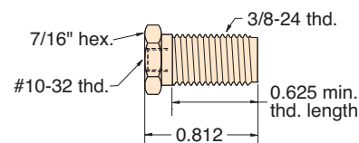
Part No. MIQC-VFT Description #10-32 Female, 3/8-24 Thd. (supplied with mounting nut and two washers)
