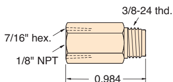
Part No. MIQC-VFP Description 1/8" NPT Female, 3/8-24 Thd.
