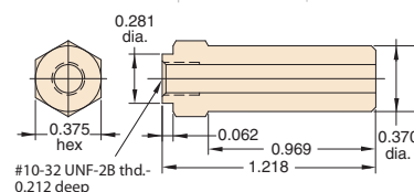
11675-12 3/8" O.D. Tube
