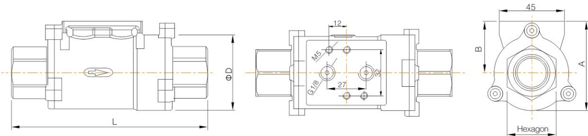
Main Dimension (201 Series)
