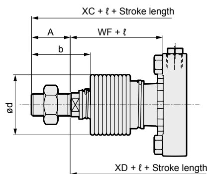
(With bellows)
