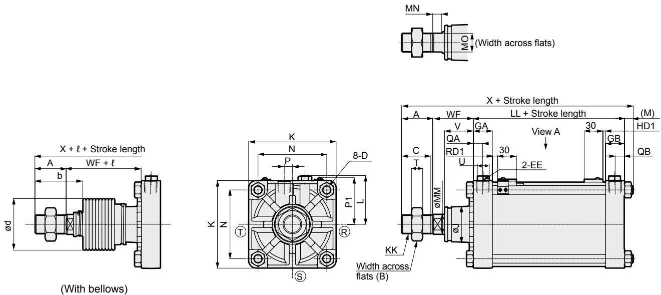
(With bellows)
