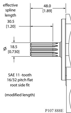
SM shaft option
